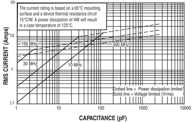
CURRENT RATING VS. CAPACITANCE ATC SERIES 100, CASE C
